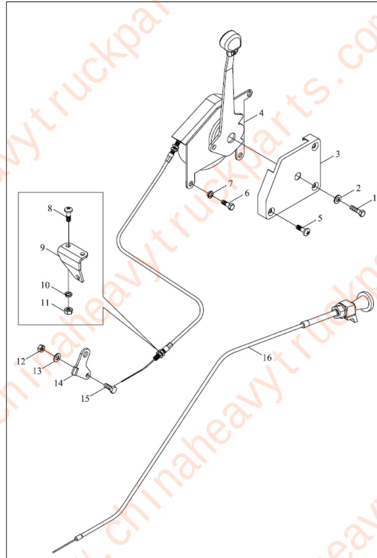
FT400.20.001 Engine control mechanism assembly-1
