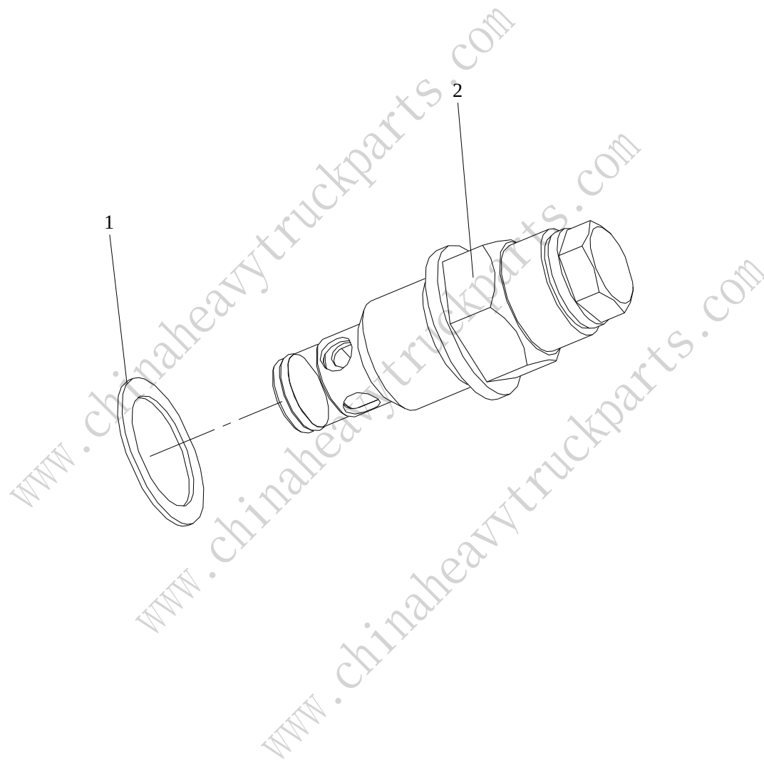
Fig. 18 Pressure regulating valve
