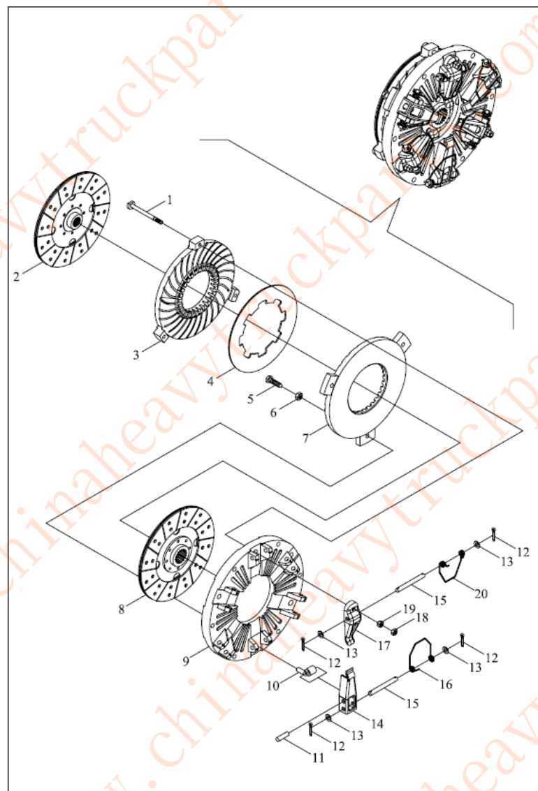
FT500A.21B.001Clutch assembly-2
