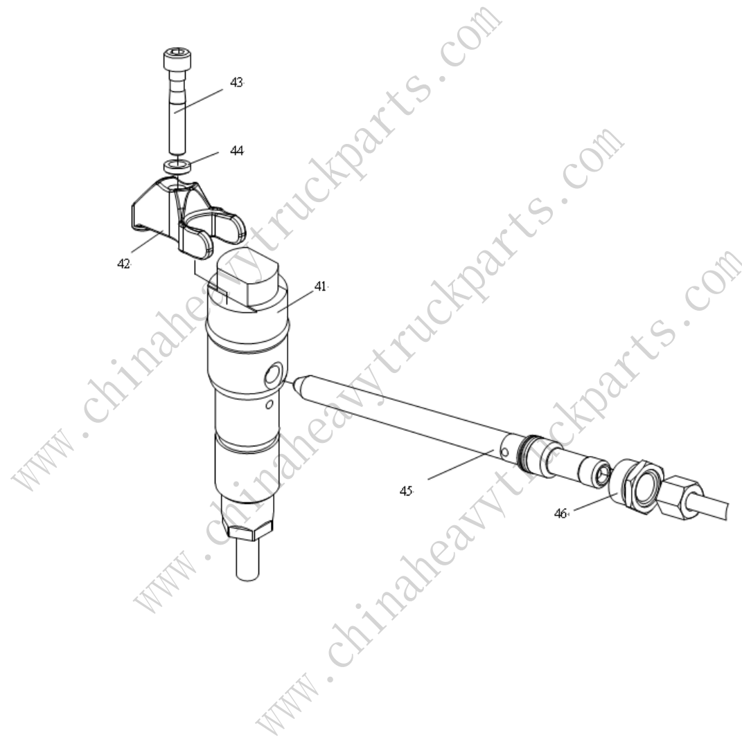
Fig. 28 Fuel supply system (V)
