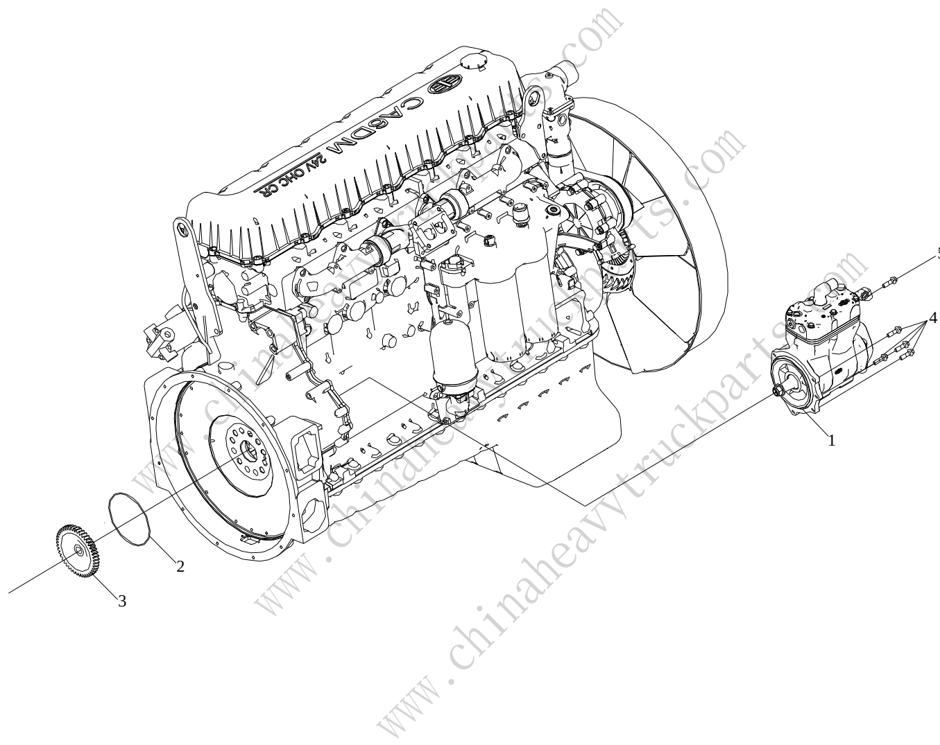
Fig. 36 Air compressor (I)
