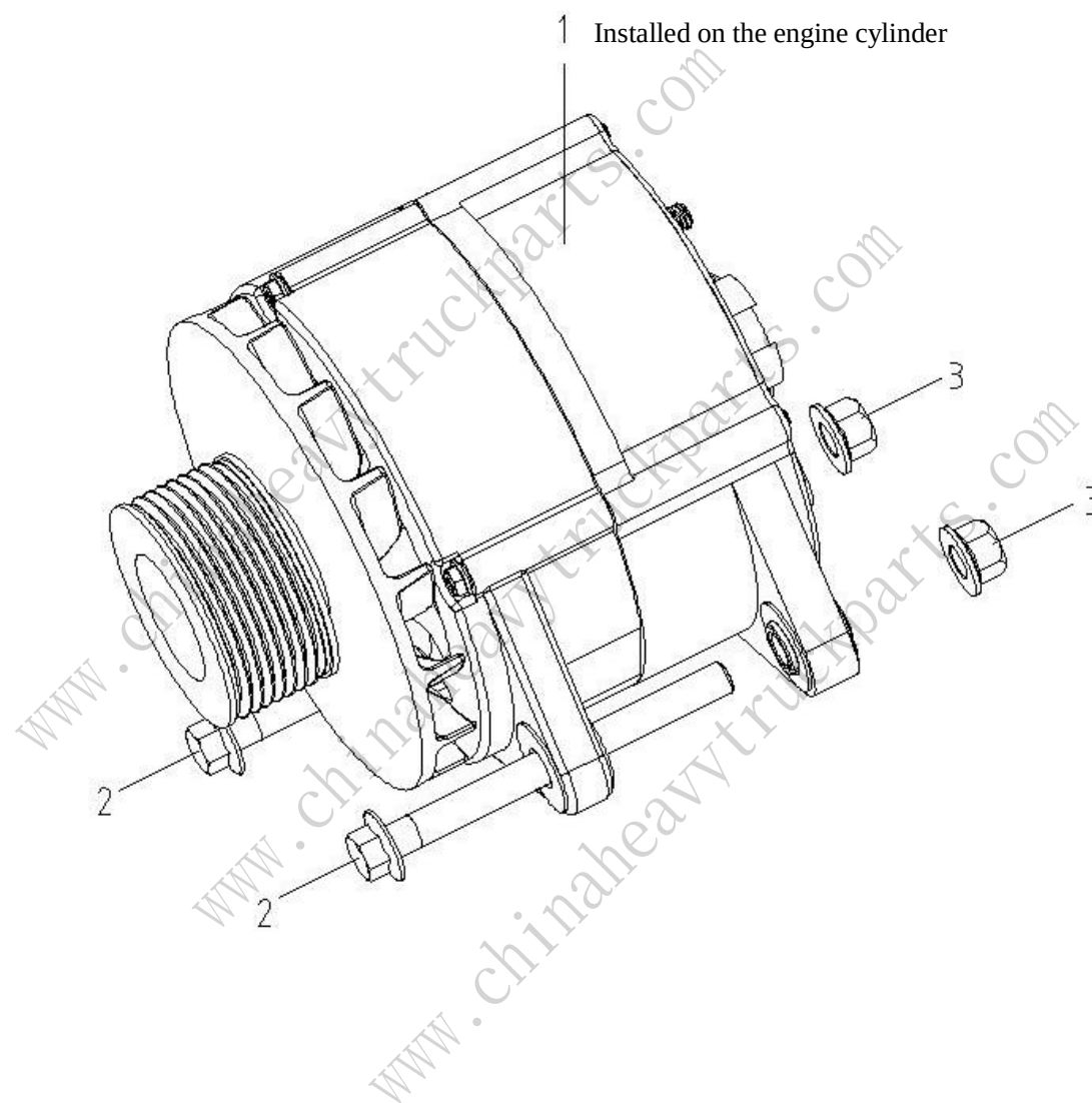
Fig. 38 Generator and connection elements
