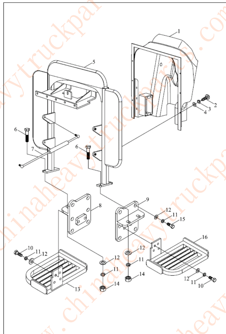
TB400B.474A Front wall fender assembly
