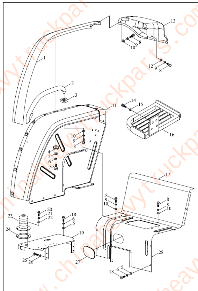
TB454.45A Floor mounting-2
