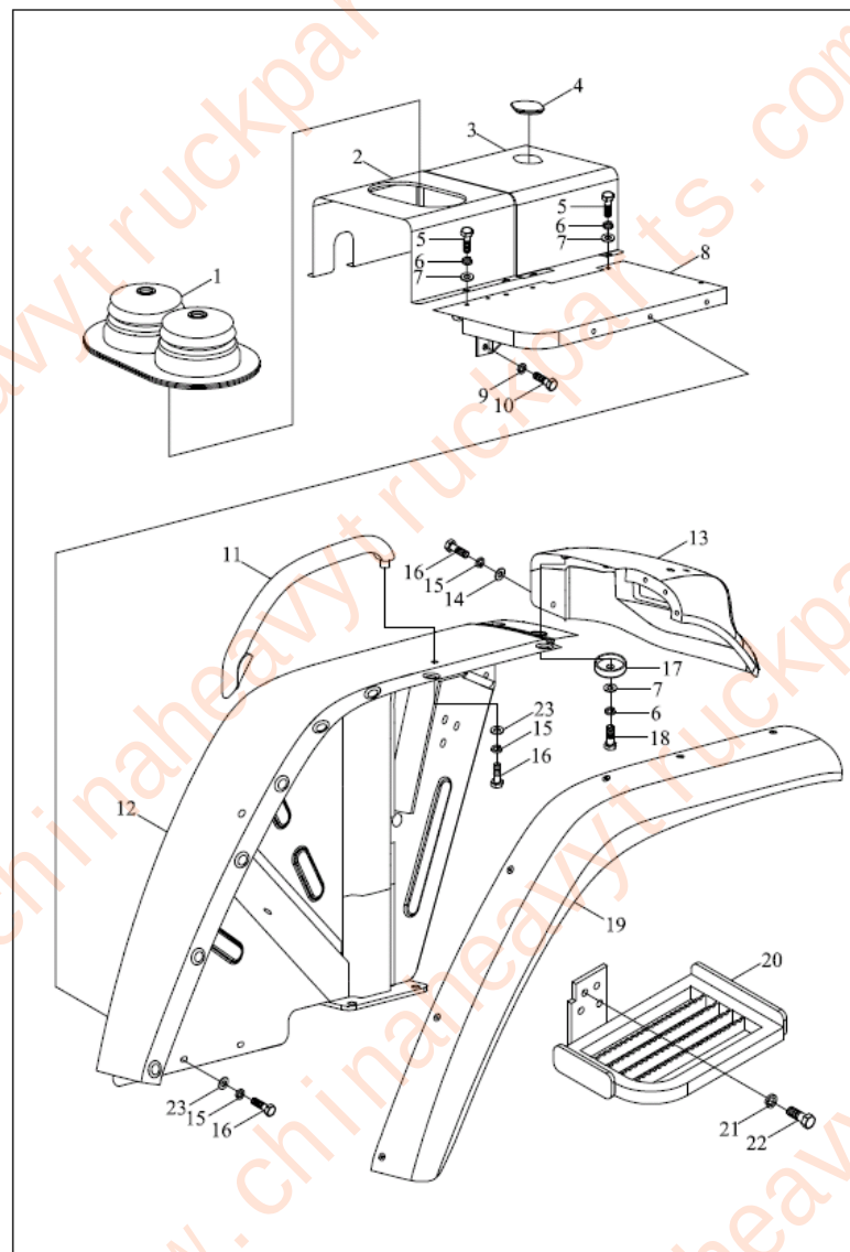
TB454.45A Floor mounting-1
