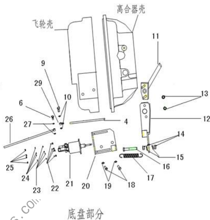
Clutch Control Mechanism on Chassis
