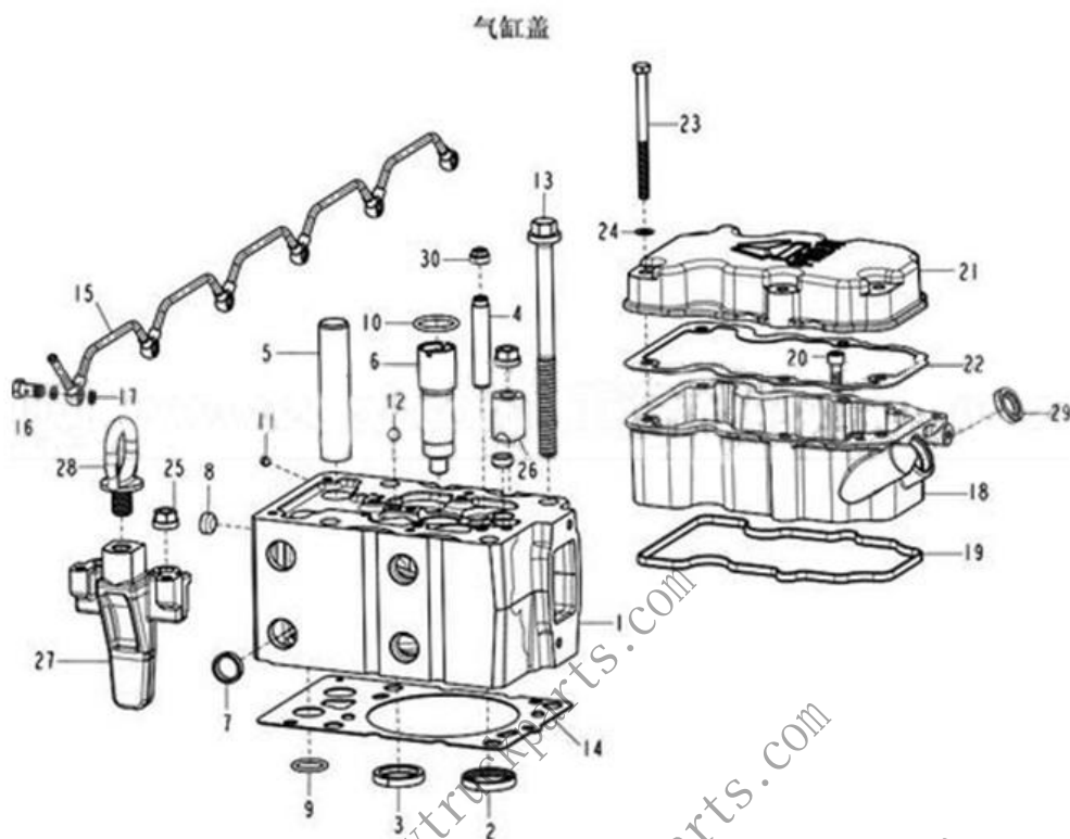
CYLINDER COVER, D12 EURO-II ENGINE
