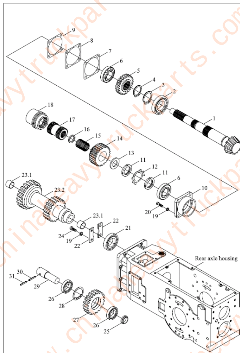
TB454.38JRear axle assembly-2
