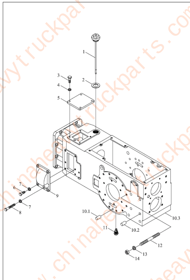
TB454.38JRear axle assembly-1
