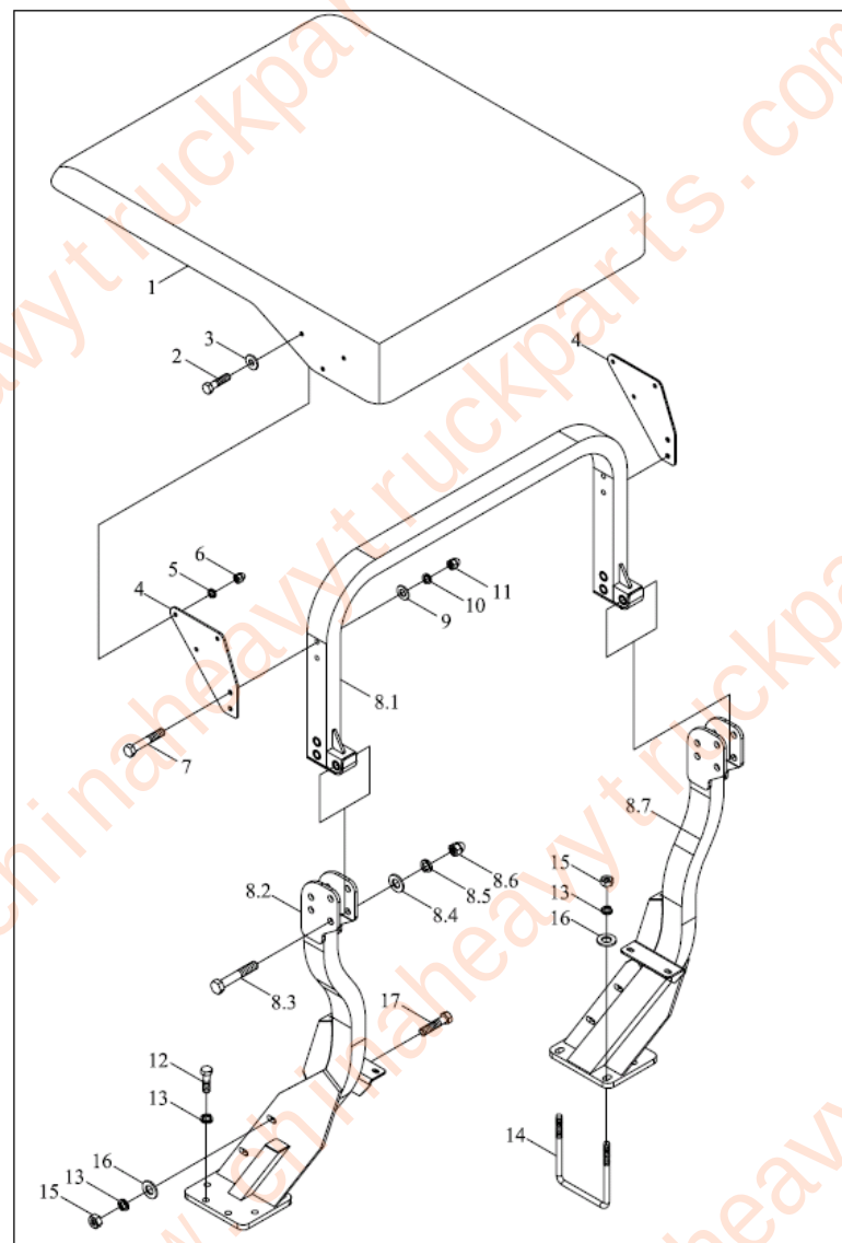
FT400.46.001 Safety frame assembly
