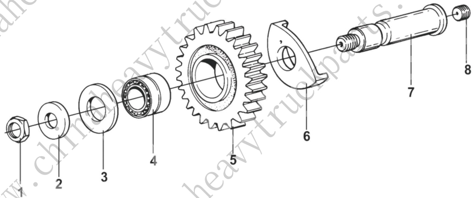
Reverse countershaft assembly
