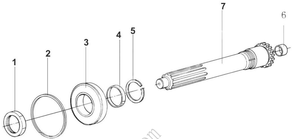
First shaft assembly
