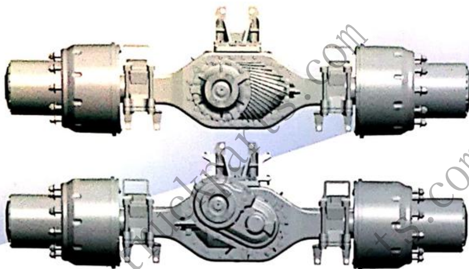
13吨/16吨中桥主减 13T/16T Medium axle final drive
