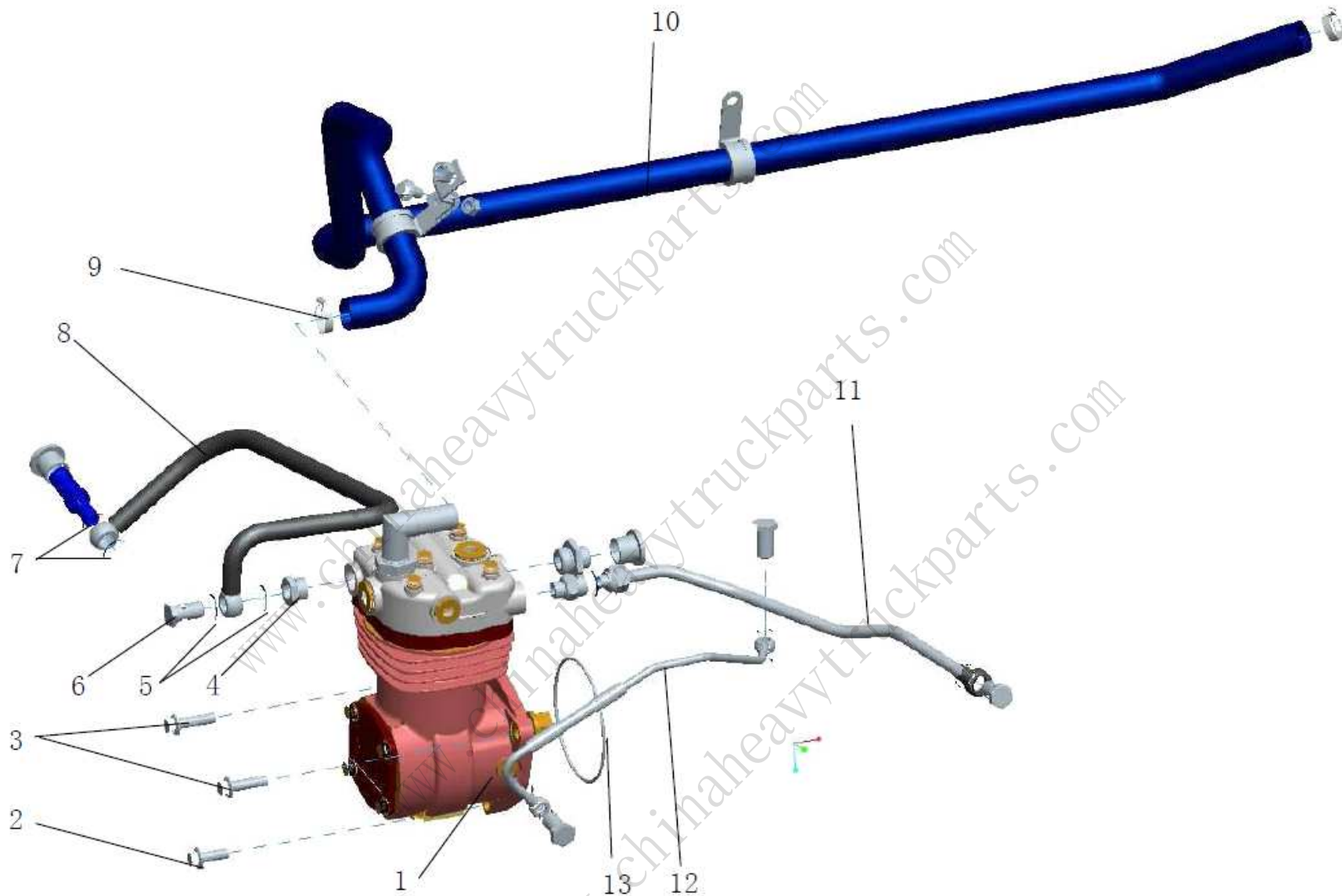
压气机管路结合组 Air compressor pipe assembly
