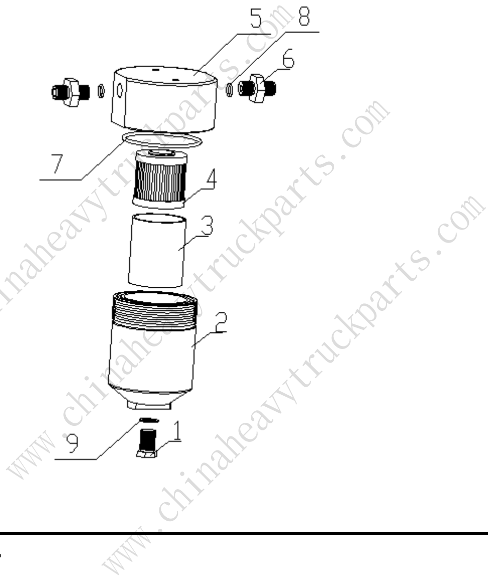
高压精滤器 high pressure fine filter
